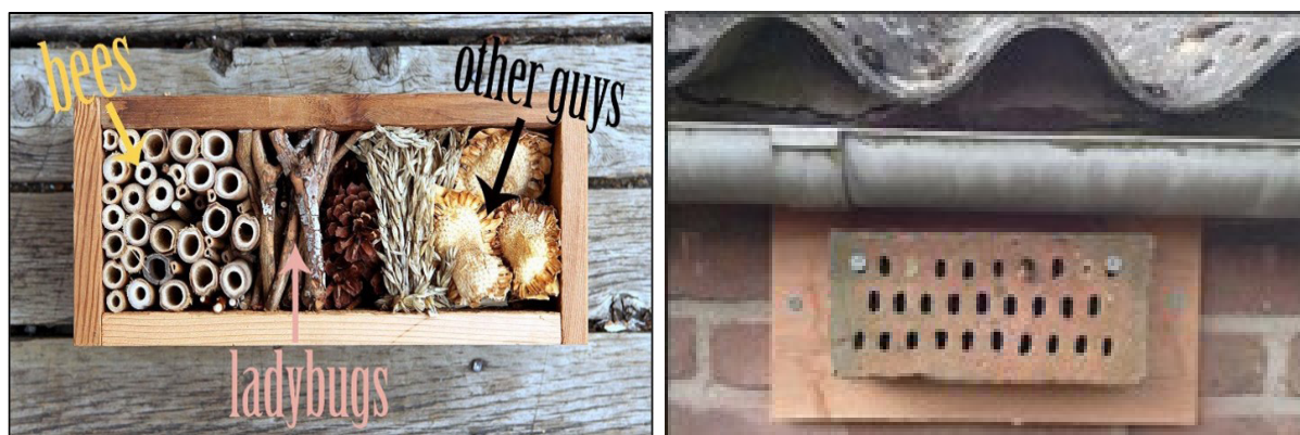
Figure 11. A design of a bee hotel, modified to create habitat for other pollinator species (left) and a brick bee hotel (right).
